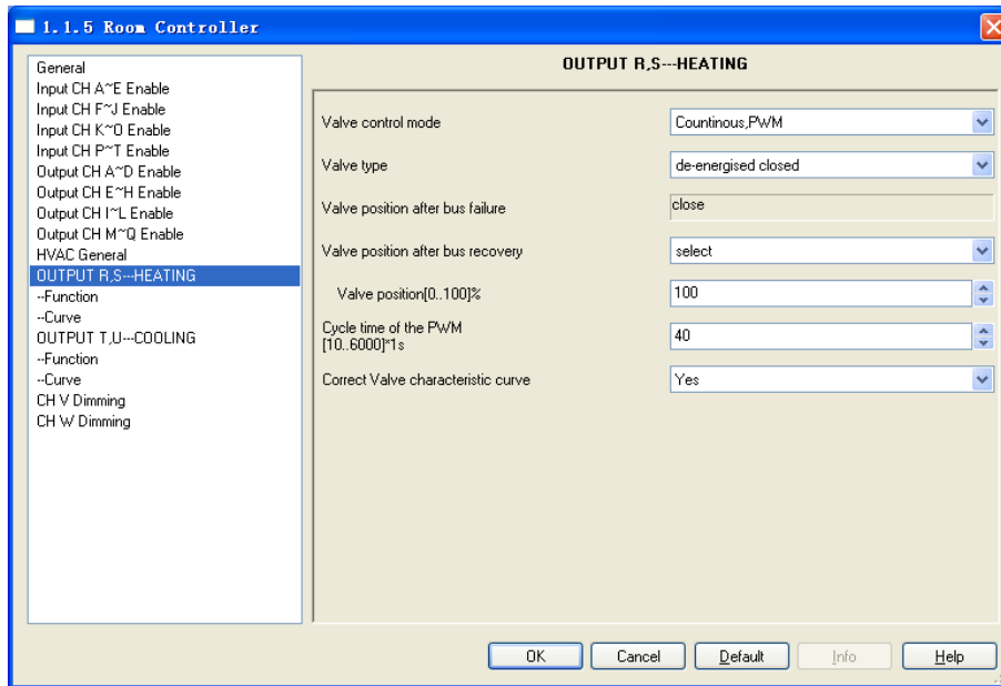
Fig. 5.35 parameter window “HEATING:Continous, PWM”
